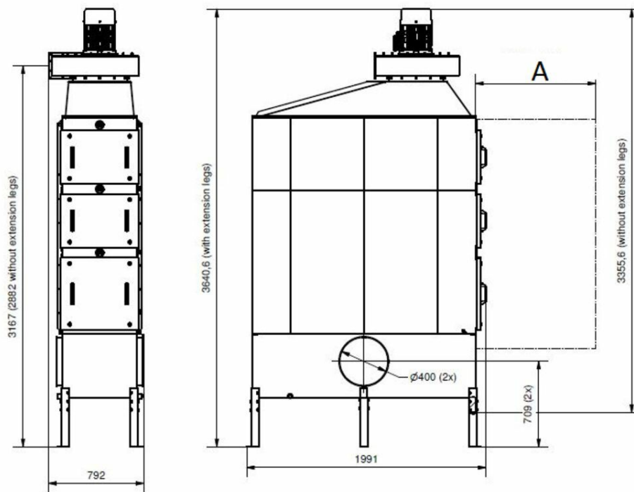
A) 1000 mm filter service space
